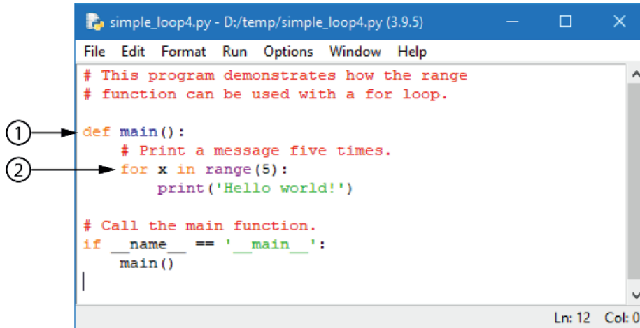
Figure B-6 Lines that cause automatic indentation
