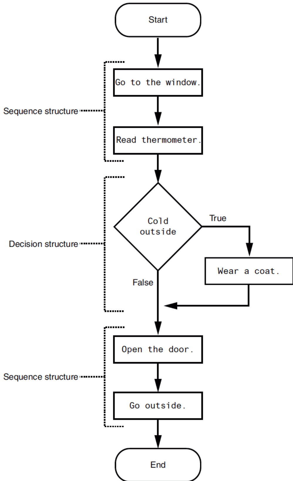
Figure 3-10 Combining sequence structures with a decision structure
