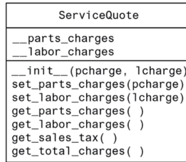
Figure 10-14 UML diagram for the ServiceQuote class
