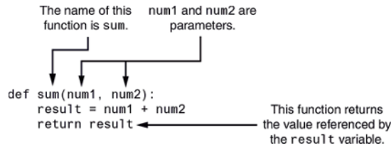
Figure 5-23 Parts of the function
