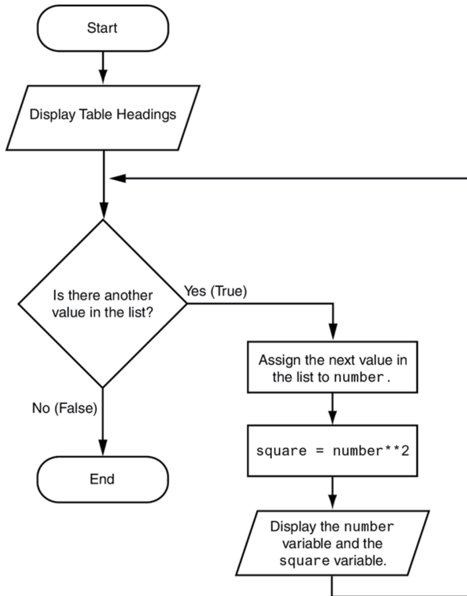
Figure 4-5 Flowchart for Program 4-8
