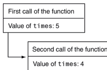
Figure 12-1 First two calls of the function
