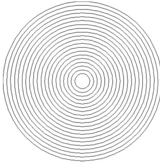
Figure 4-10 Concentric circles
