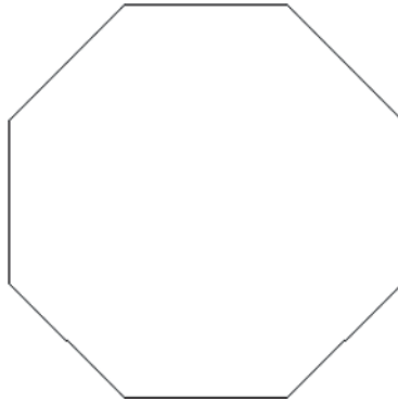
Figure 4-9 Octagon
