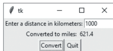
Figure 13-27 The window showing 1000 kilometers converted to miles
