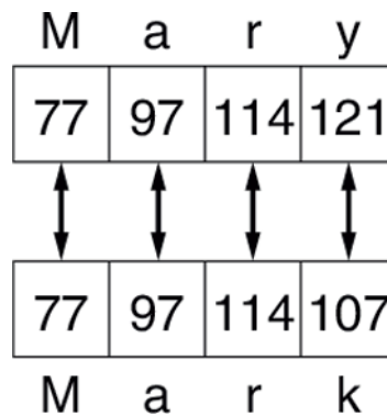
Figure 3-9 Comparing each character in a string
