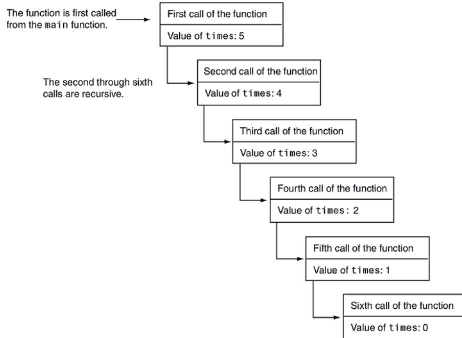
Figure 12-2 Six calls to the message function
