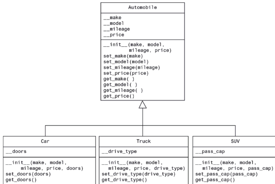
Figure 11-2 UML diagram showing inheritance
