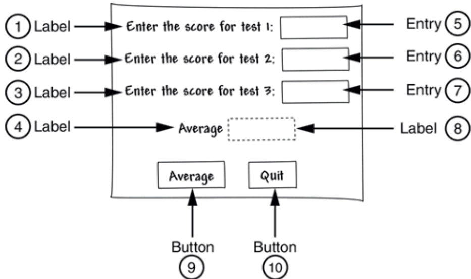
Figure 13-29 A sketch of the window
