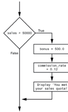
Figure 3-4 Example decision structure
