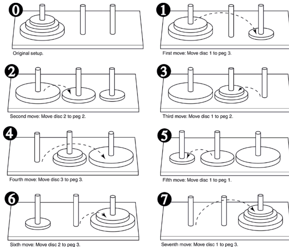
Figure 12-6 Steps for moving three pegs
