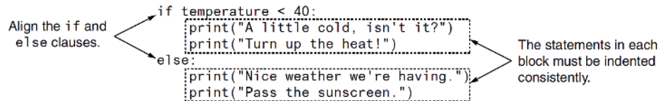
Figure 3-7 Indentation with an if-else statement
