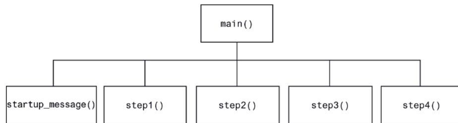
Figure 5-11 Hierarchy chart for the program
