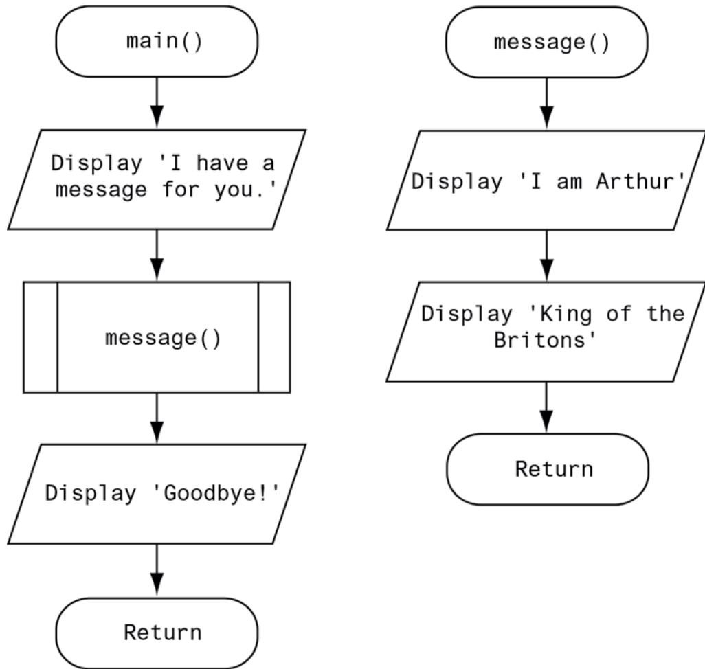
Flowchart for Program 5-2
