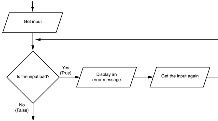
Figure 4-7 Logic containing an input validation loop
