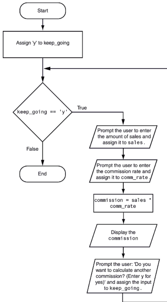
Figure 4-3 Flowchart for Program 4-1
