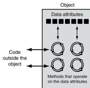
Figure 10-2 Code outside the object interacts with the object's methods
