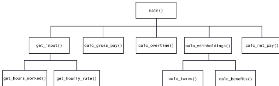
Figure 5-10 A hierarchy chart
