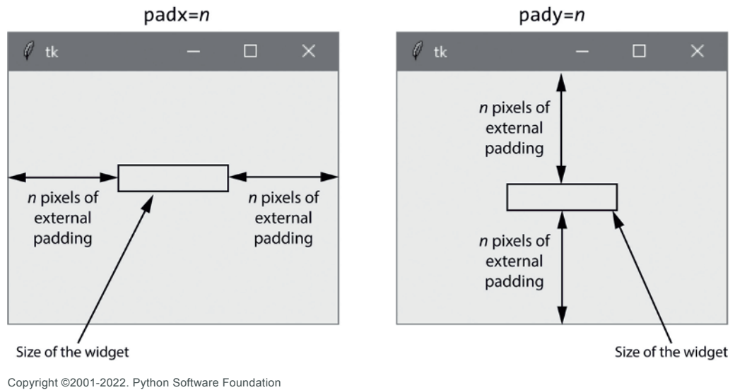
Figure 13-15 Horizontal and vertical external padding
