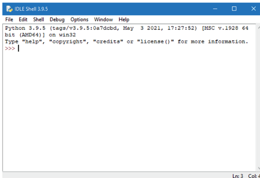
Figure 1-20 IDLE
