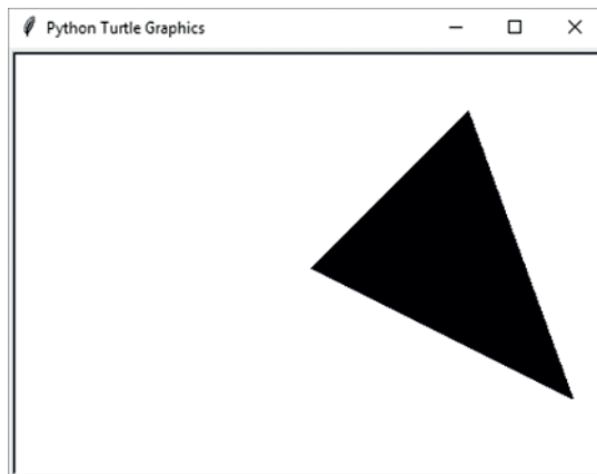
Figure 2-27 Shape filled
