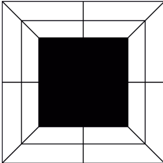
Figure 5-31 Rectangular pattern
