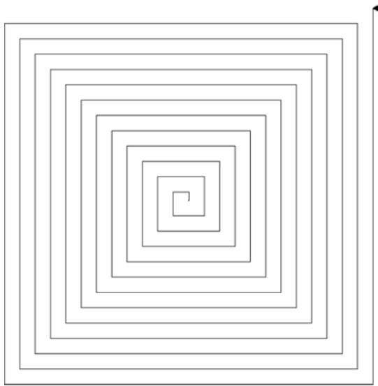
Figure 4-15 Hypnotic pattern
