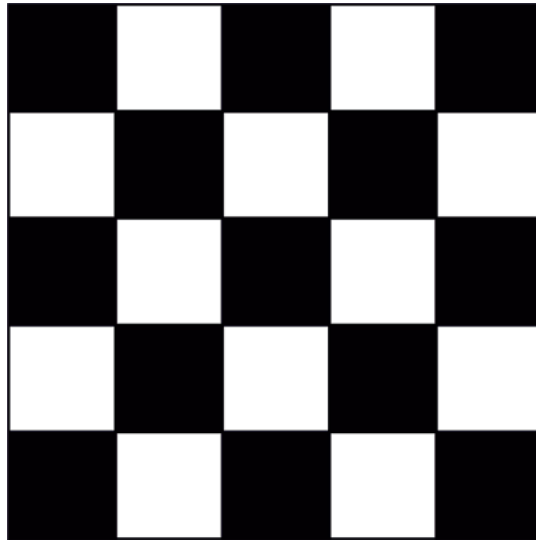
Figure 5-32 Checkerboard pattern
