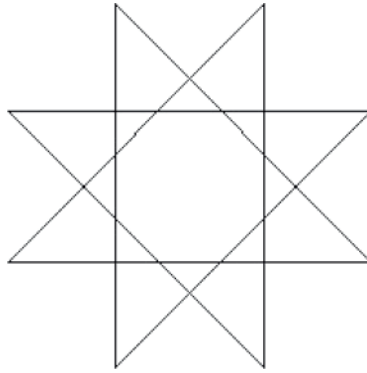
Figure 4-14 Star pattern
