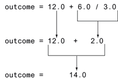
Figure 2-9 Operator precedence
