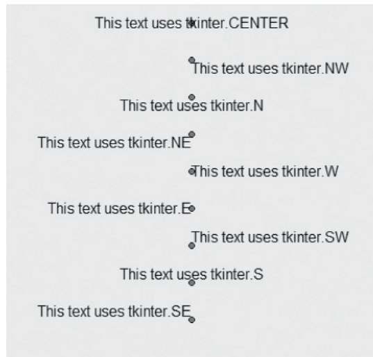
Figure 13-59 Results of the various anchor values
