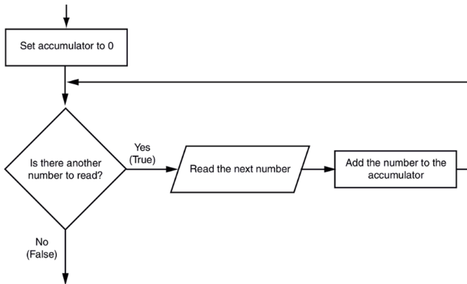
Figure 4-6 Logic for calculating a running total
