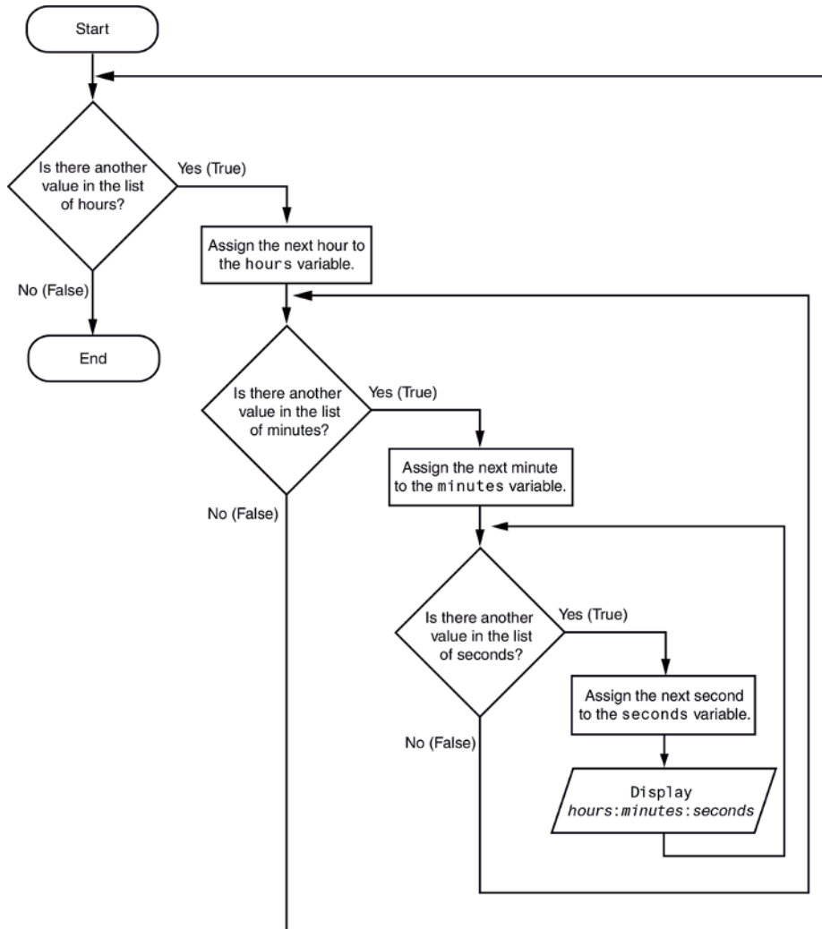
Figure 4-8 Flowchart for a clock simulator
