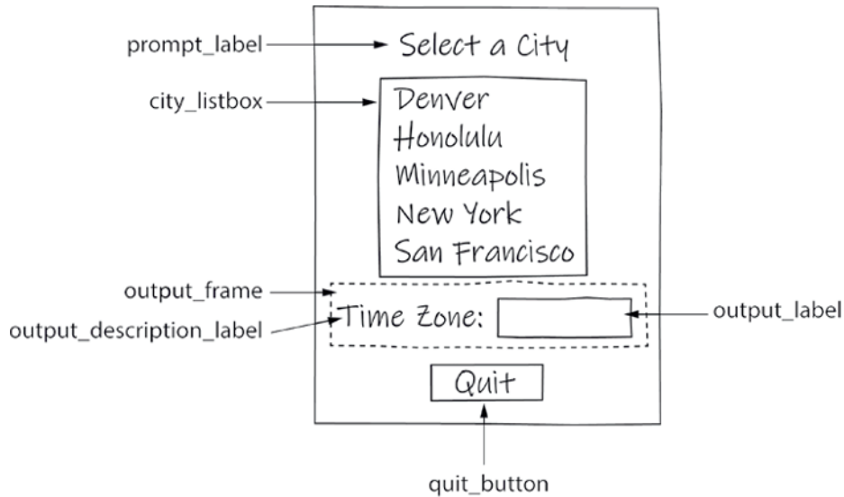
Sketch of the Time Zone Program
