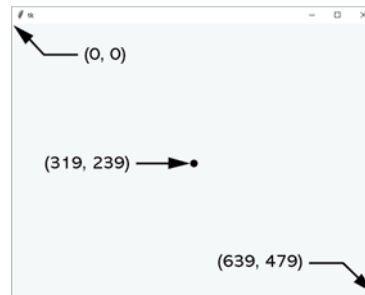
Figure 13-45 Various pixel locations in a 640 by 480 window
