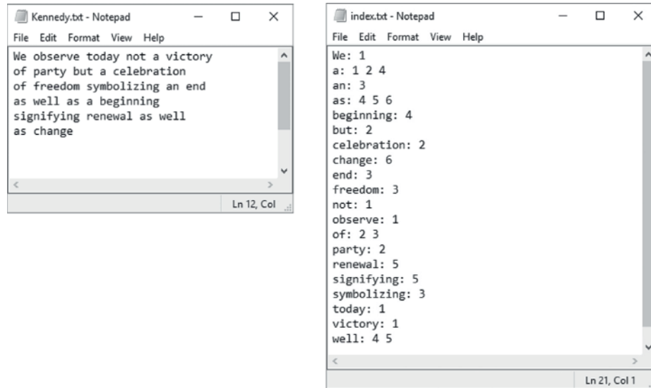
Figure 9-2 Example of original file and index file
